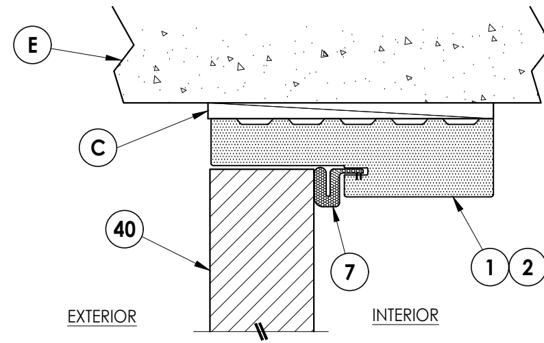
3 VERTICAL CROSS SECTION 6 Outswing Shown (Inswing Similar) Shown Direct to Masonry
