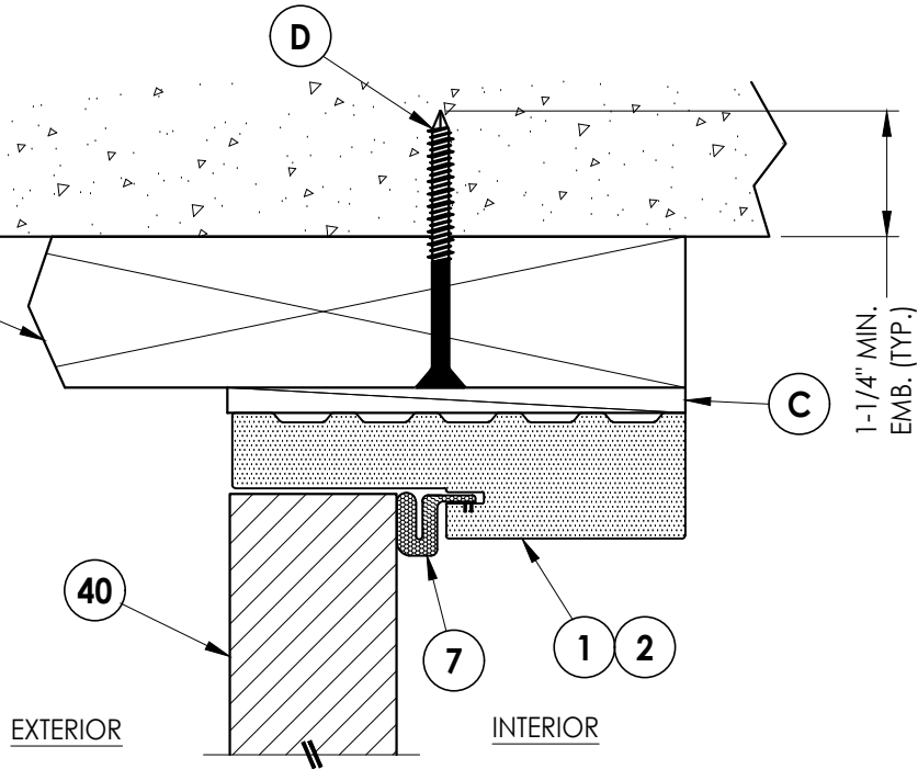
3 4 VERTICAL CROSS SECTION Outswing Shown (Inswing Similar) Shown w/ 2X Buck
