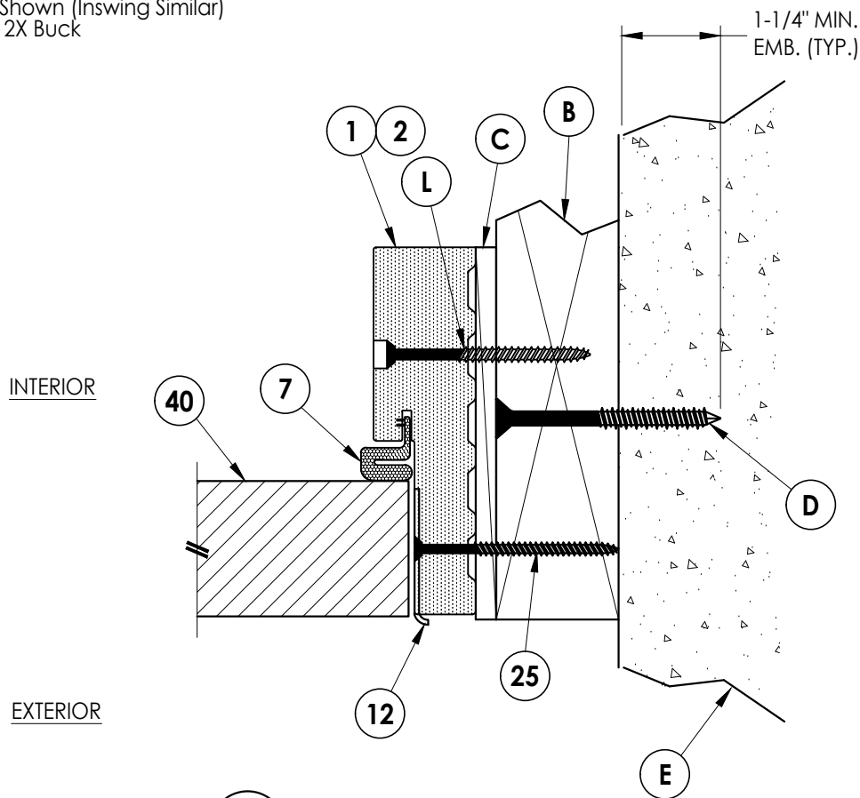
2 4 HORIZONTAL CROSS SECTION Outswing Shown (Inswing Similar) Shown w/ 2X Buck
