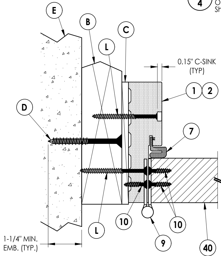
1 4 HORIZONTAL CROSS SECTION Outswing Shown (Inswing Similar) Shown w/ 2X Buck
