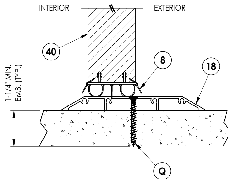
3 VERTICAL CROSS SECTION 7 ADA Sill
