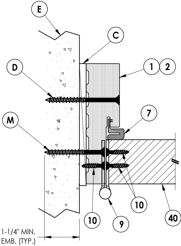
1 HORIZONTAL CROSS SECTION 6 Outswing Shown (Inswing Similar) Shown Direct to Masonry
